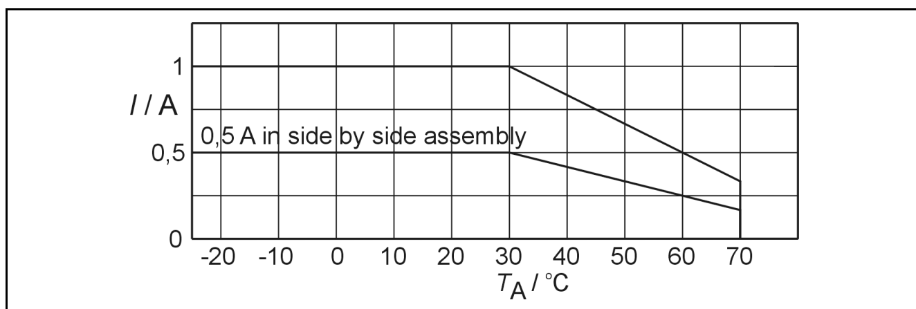
Derating curve for SLO A230TR.
