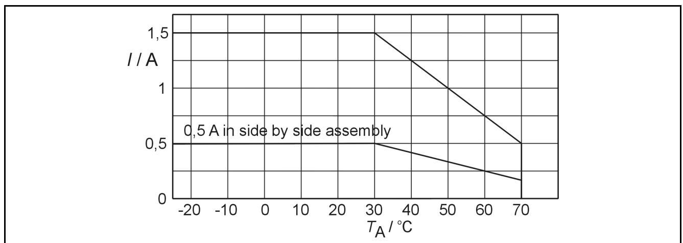
Derating curve for SLO P230TR.
