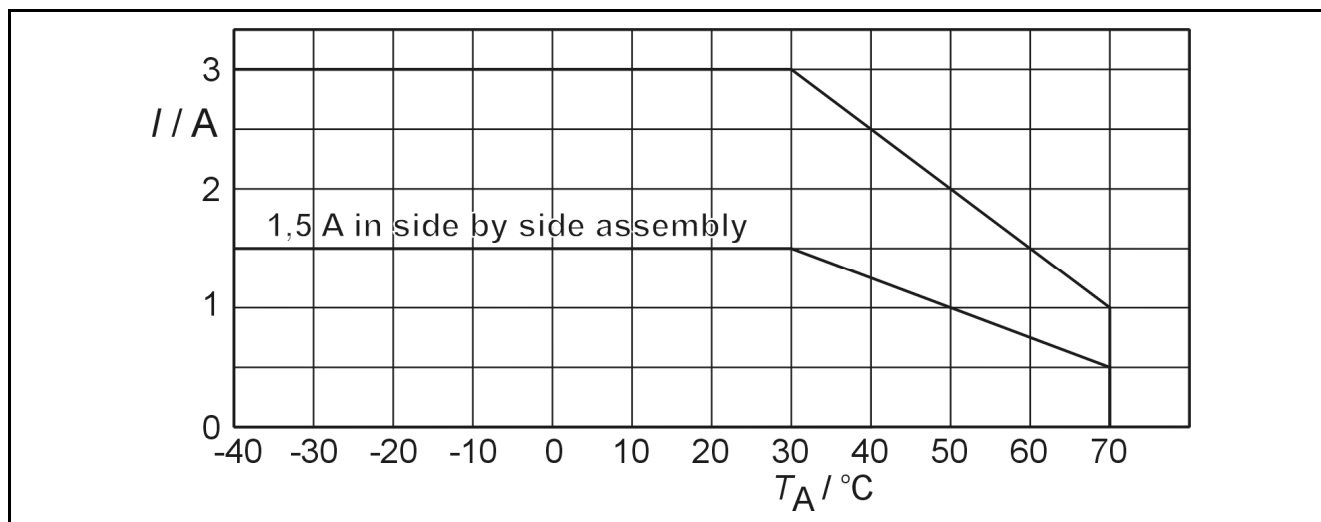
Derating curve for SLO 24TH.
