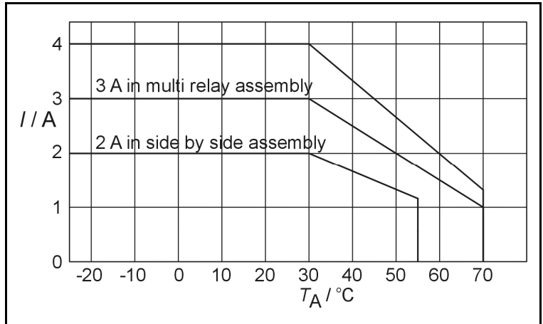
Derating curve for EXO 220CHA4.
