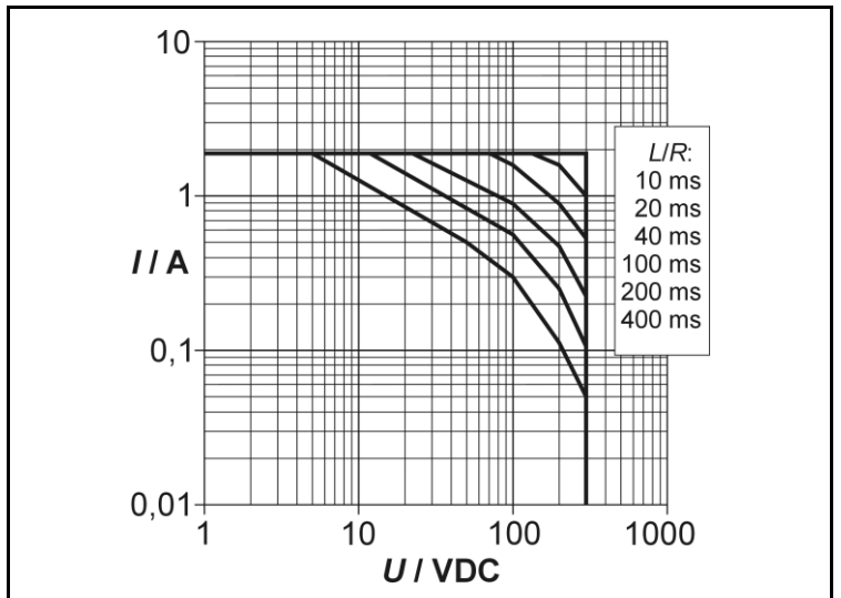
Derating curve for inductive loads.
